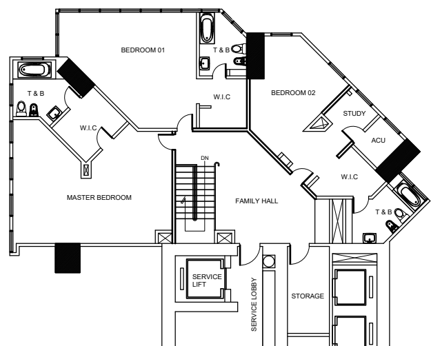
39TH FLOOR (UNIT-A)
